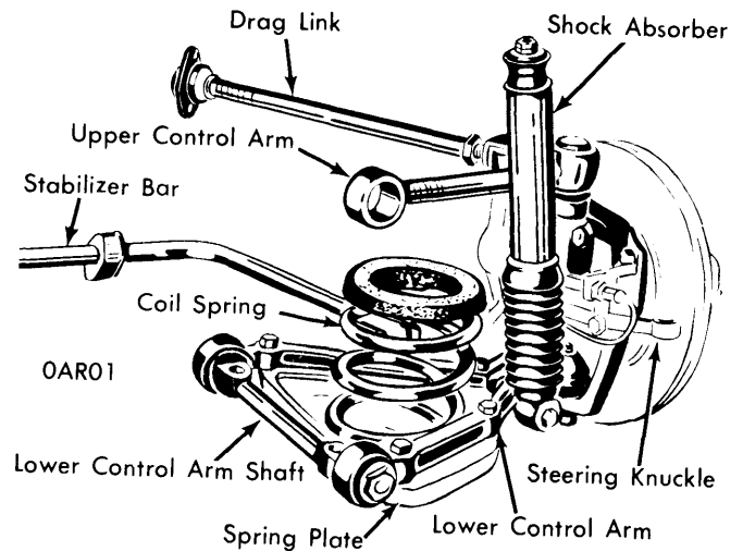
ALFA ROMEO GIULIA, 1750 & 2000 FRONT SUSPENSION COMPONENTS
