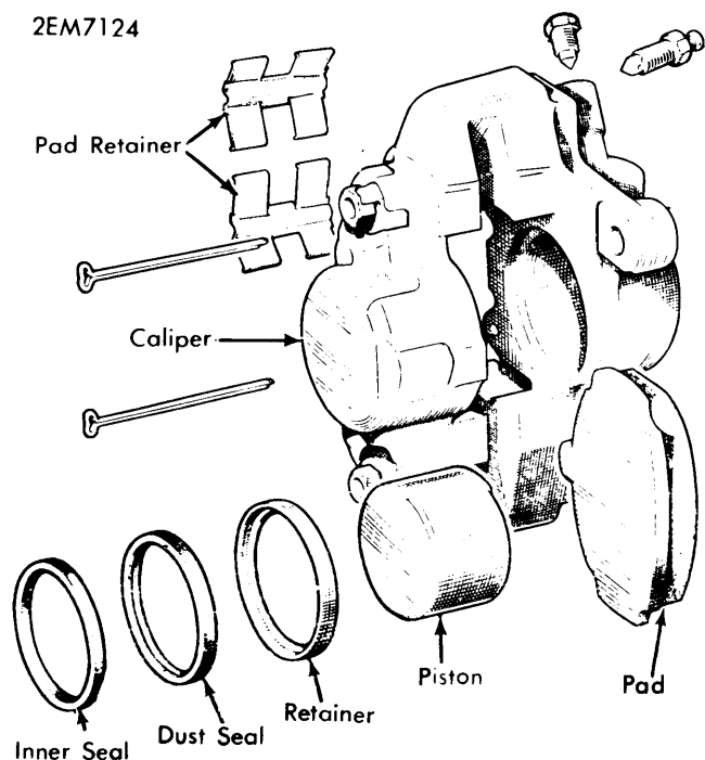
BRAKE CALIPER
