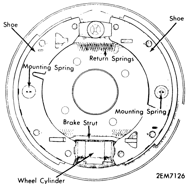
DRUM BRAKE ASSEMBLY
