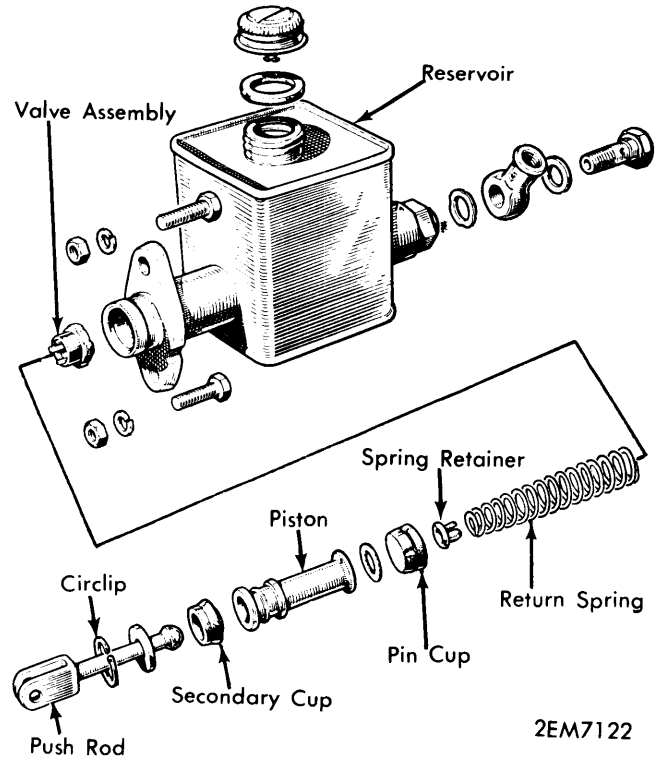
MASTER CYLINDER (SINGLE)
