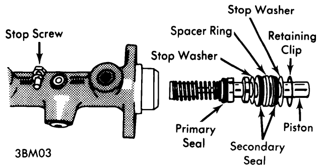
PRIMARY PISTON ASSEMBLY
