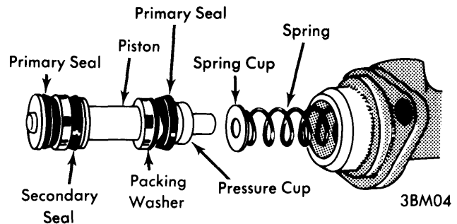
SECONDARY (FRONT) PISTON ASSEMBLY
