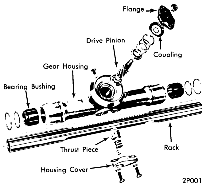
RACK & PINION ASSEMBLY
