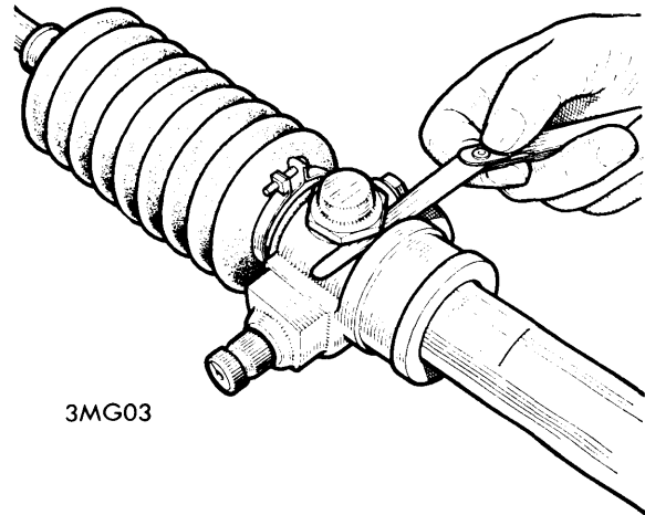
CHECKING RACK DAMPER CAP CLEARANCE
