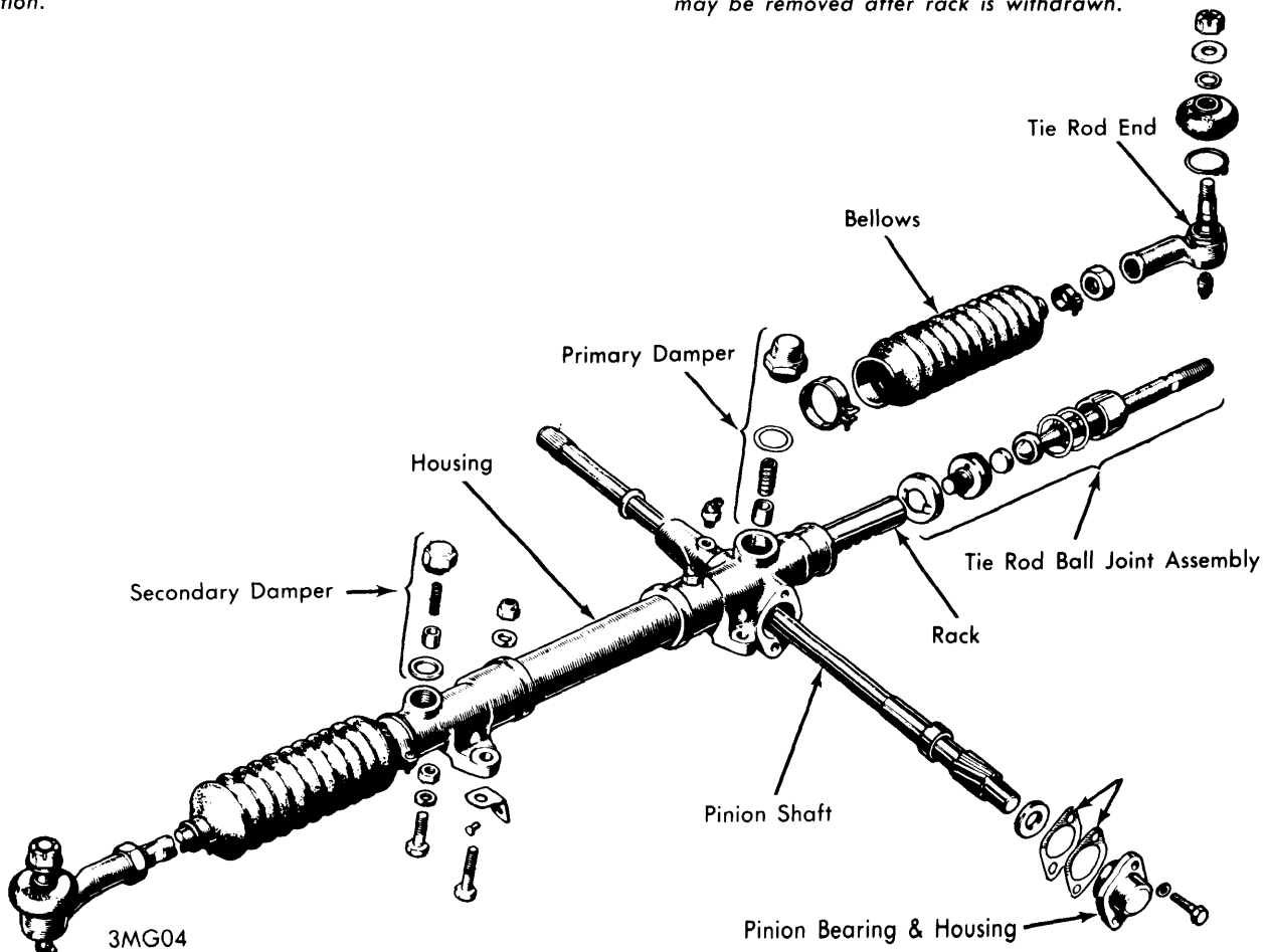
MG MIDGET RACK &amp; PINION
