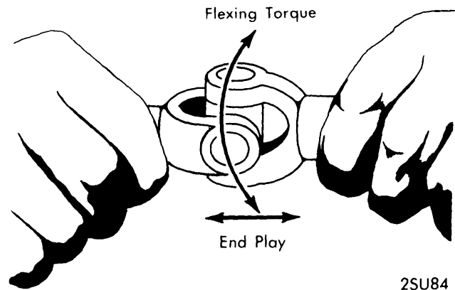
UNIVERSAL JOINT
