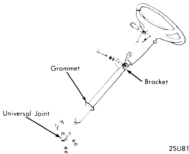
STEERING COLUMN ASSEMBLY
