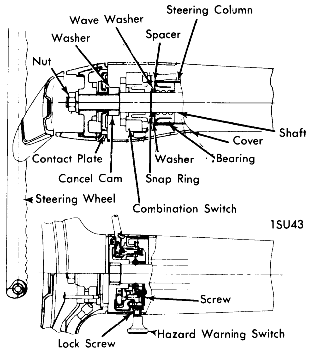
STEERING WHEEL & UPPER ASSEMBLY
