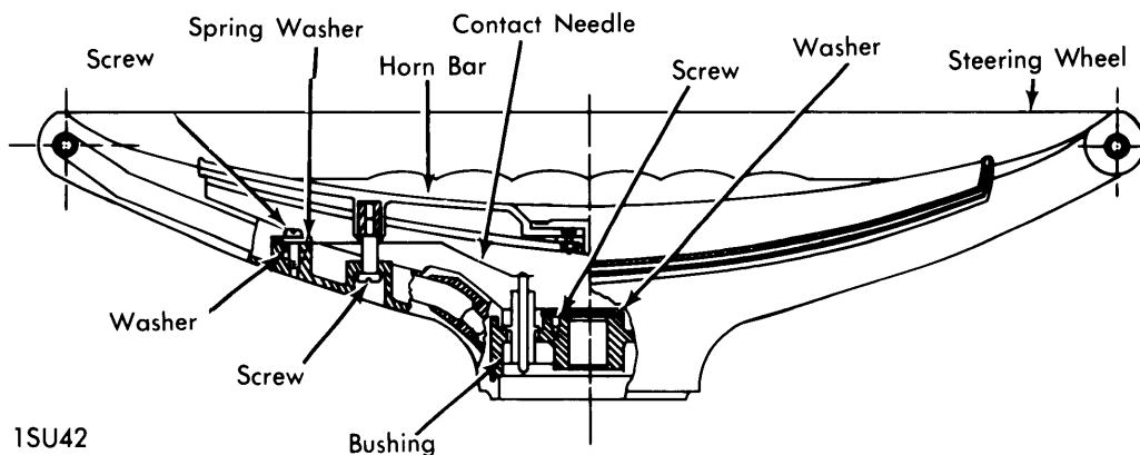
STEERING WHEEL ASSEMBLY
