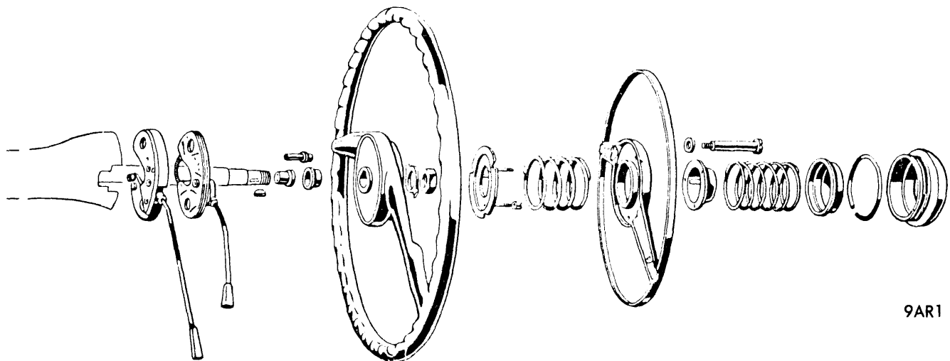
STEERING WHEEL ASSEMBLY
