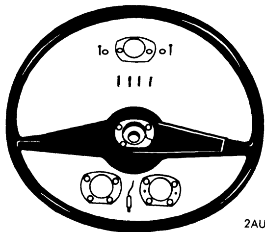
STEERING WHEEL COMPONENTS
